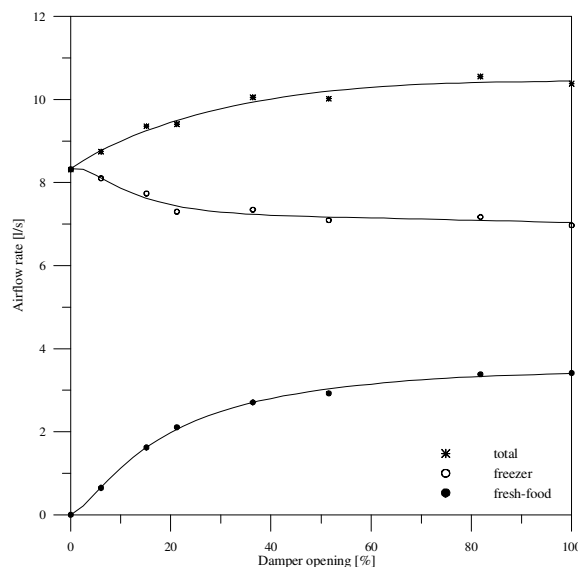
Figure 8. Airflow as a function of damper position.
